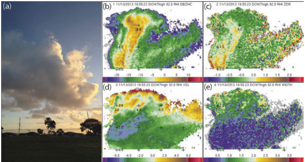
FIG. 9. Cumulus cloud observations on 13 Nov. (a) Photo of the cloud at 1655 UTC, (b) radar reflectivity (dBZ), (c) differential reflectivity Z_{DR} (dB), (d) Doppler velocity ( \text{m s}^{-1} ), and (e) spectrum width ( \text{m s}^{-1} ). Tick marks denote 1 km in the vertical and in the horizontal. The radar is at the bottom-left corner of each panel, and the RHIs are at 92^\circ relative to the truck ( 57^\circ heading).
